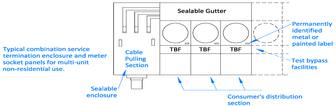
Figure 9.14.3 – Acceptable Multiple Meter Socket Installations - Miscellaneous Configurations
