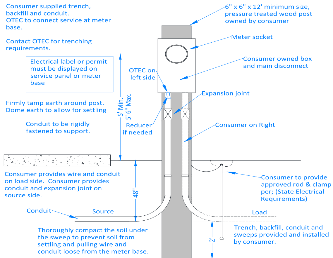
Figure 9.10.1 - POST-MOUNTED INSTALLATIONS
