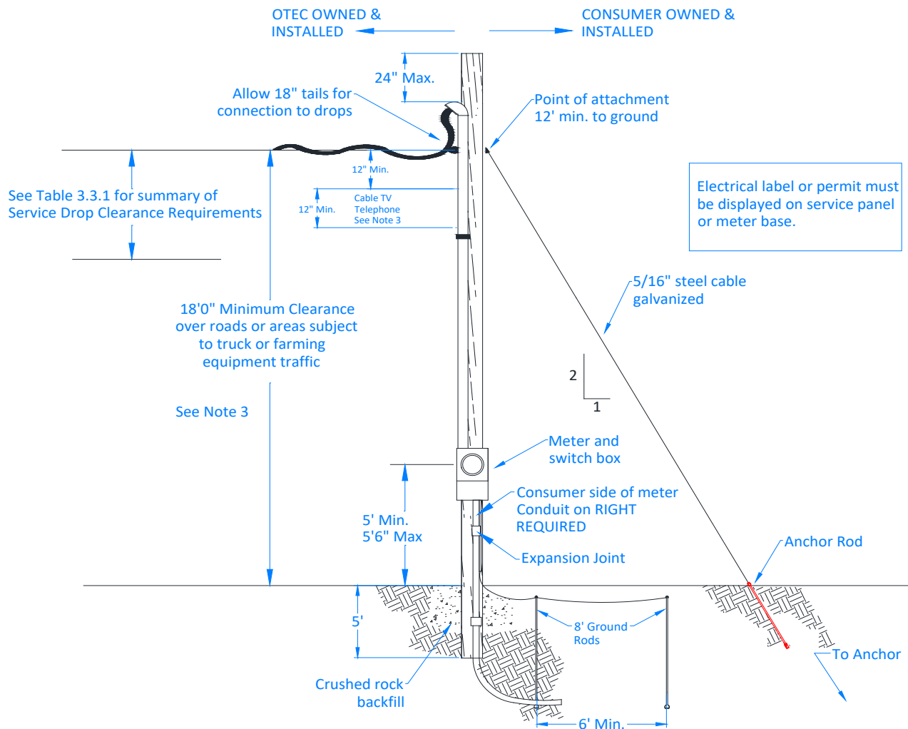
Figure 9.7.1 – Overhead Service to Underground Consumer Side
