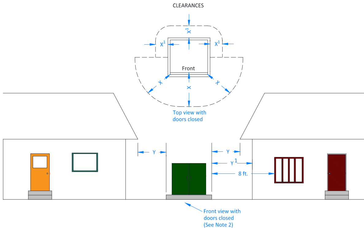
Figure 9.17.1 – Pad Mounted Transformer Minimum Clearance Requirements
